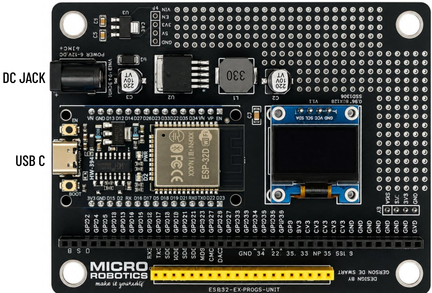
Fully Assembled ESP32 IOT Controller
